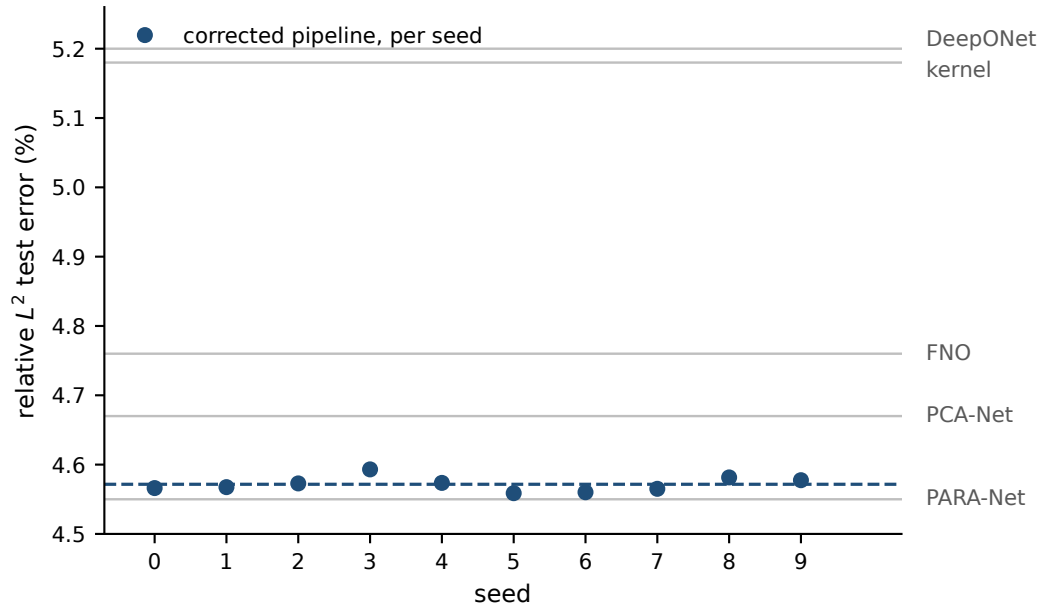
Structural mechanics: ten seeds
