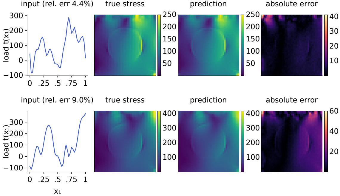
Figure 1: Example predictions of the full pipeline. Top: a median-error test case; bottom: a case at the 98th error percentile. Columns: input load, true von Mises stress, prediction, and pointwise absolute error; the error panels use a smaller scale. Errors concentrate in the high-traction corner, as also reported by Mora et al. (2025).
