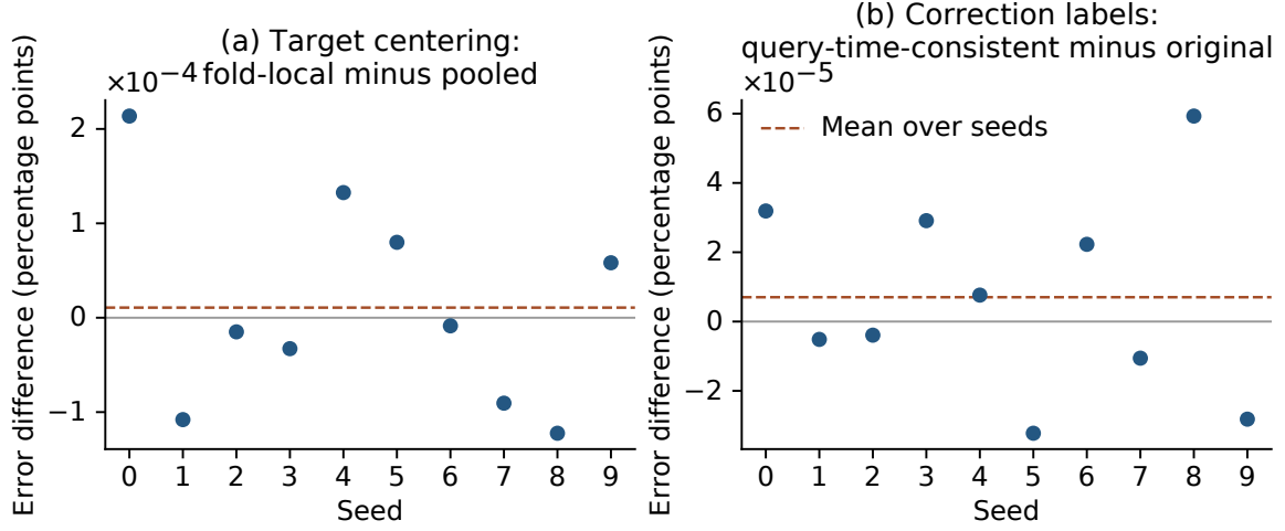
Figure 2: Paired changes in mean relative test error for the ten mechanics seeds. Left: fold-local minus pooled target centering, with downstream refiner training and fitting repeated in both arms. Right: correction labels consistent with the query-time mean minus the original labels, with the mean and kernel fixed. Positive values mean higher error after the change. The panels use separate vertical scales. All points use the same public test block; the dashed lines are seed means.
