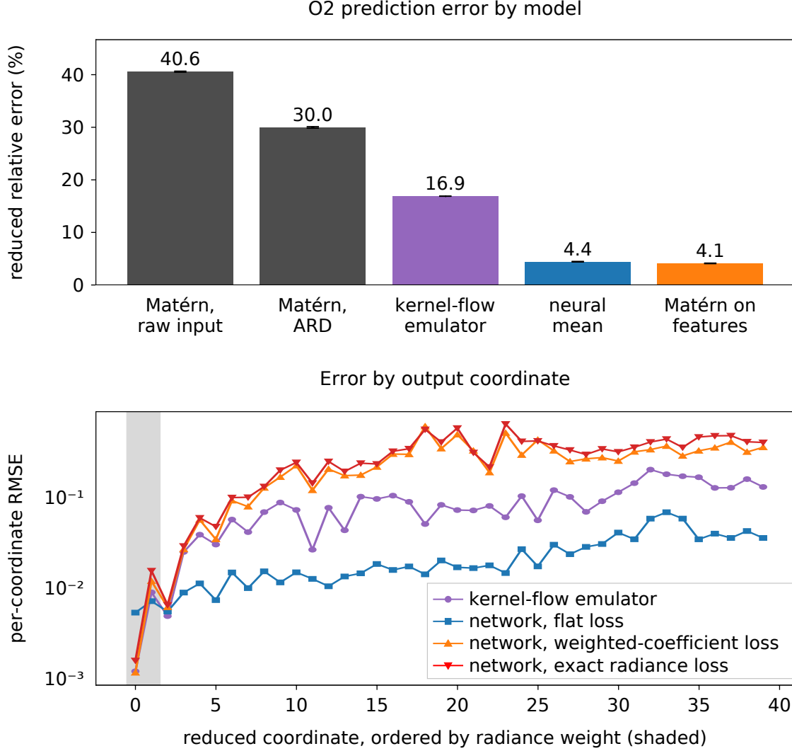
Figure 3: O2 results over ten seeds. Upper panel: reduced error for the representation comparison; bars and error bars are seed means and standard deviations. Exact Matérn regression has 40% error on raw inputs and 4.1% on the trained network’s features; the kernel-flow emulator and the network have intermediate reduced errors. Lower panel: per-coordinate test RMSE averaged over seeds, with coordinates ordered by their radiance weight (shaded). Networks are named by their training loss. The coordinate combination selects each output by validation RMSE.
