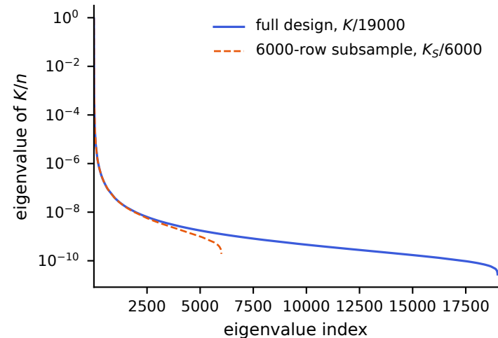
Matern spectrum, normalized by n
