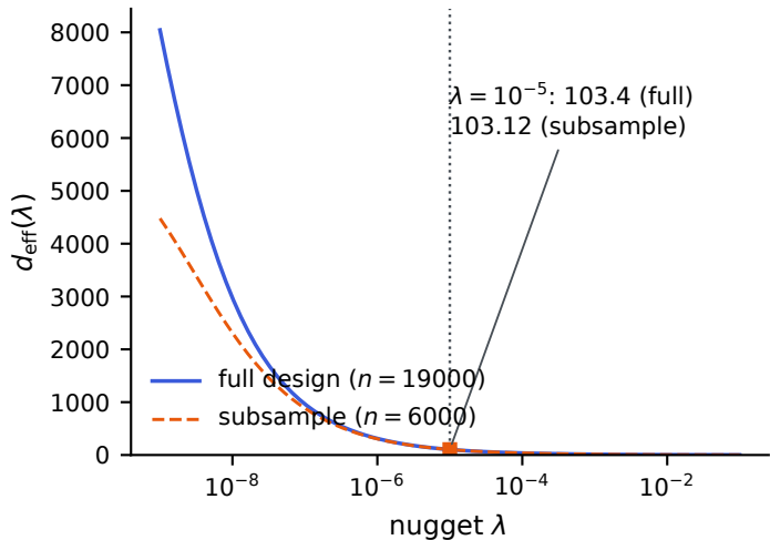
Effective dimension of the smoother
