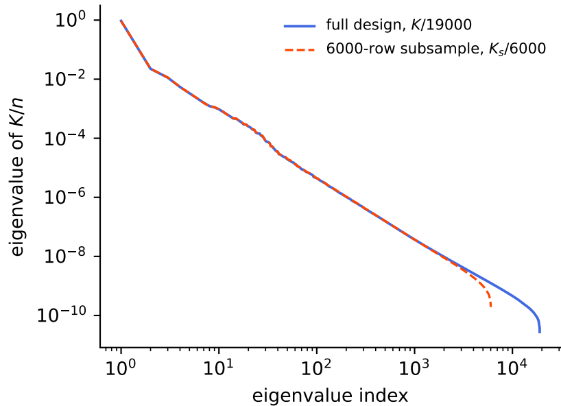
Matern spectrum, normalized by n
