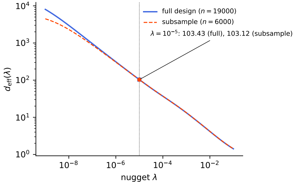
Effective dimension of the smoother
