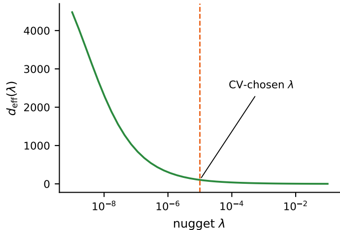
effective dimension (Lemma S5.1 identity)
