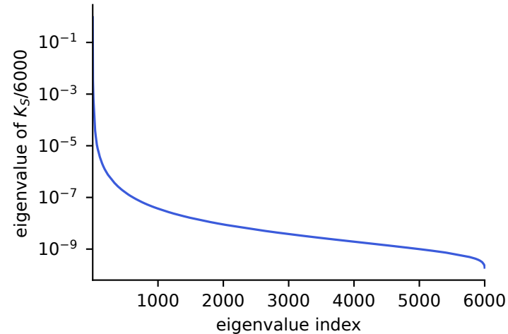
Matérn spectrum: 6000 selected rows
