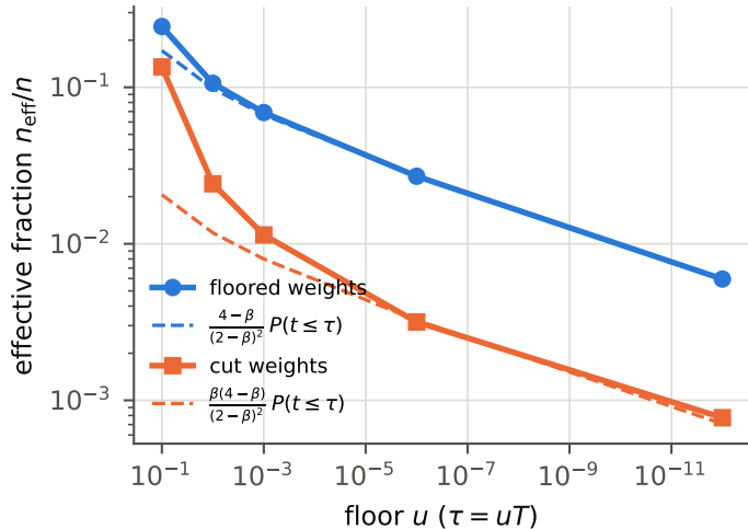
(a) effective sample size
