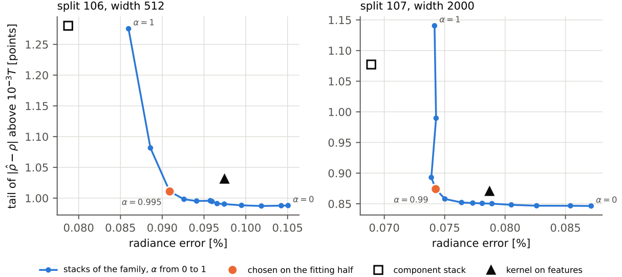
Figure 2: Stacks of the family of Proposition 6.12 on one held-out half of two EMIT runs, from the first-order retrieval error ( \alpha = 0 ) to the forward error at \rho = 0.7 ( \alpha = 1 ): the radiance error against the 95th percentile of the retrieval error on the physical domain above 10^{-3}T_{\text{train}} . The orange point is the stack whose \alpha is chosen on the other half; the square is the component stack and the triangle the kernel on learned features.
