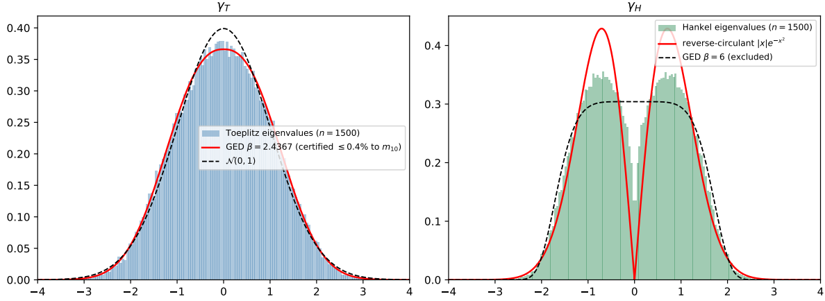
Figure 1: Simulated spectral densities ( n = 1500 , 60 repetitions). Left: \gamma_T with the GED surrogate ( \beta = 2.4367 ; indistinguishable at this resolution, provably distinct at order 6) and the standard Gaussian. Right: \gamma_H (bimodal) with the reverse-circulant density |x|e^{-x^2} and the excluded GED fit.
