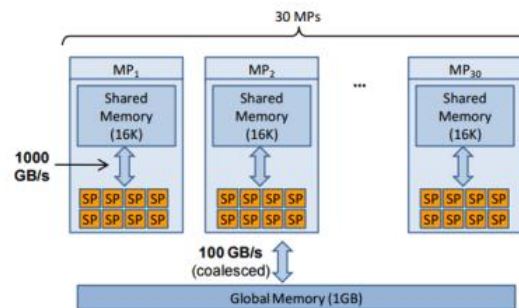
Figure 1. Simplified schematic for the Nvidia GeForce GTX 280 graphics card, with 240 total cores (30 multi-processors with 8 stream processors each).
