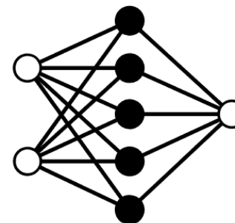
classifier
