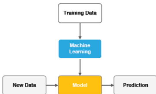
Machine learning
