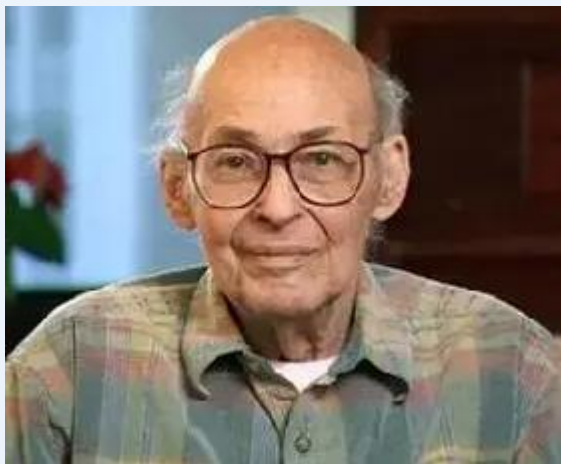
Minsky
