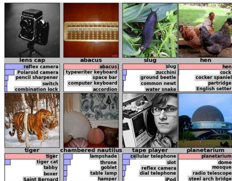
Validation classification
