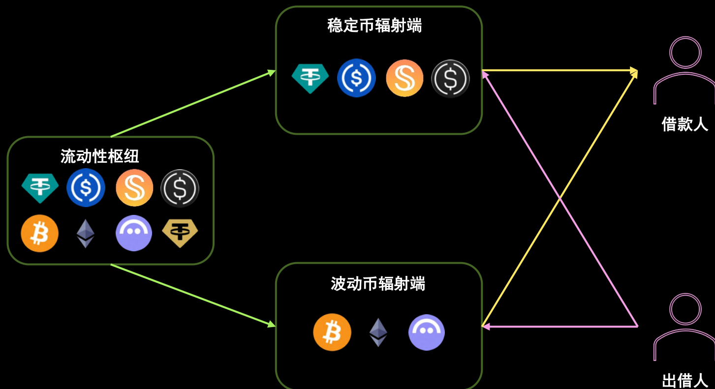
Aave V4 Architecture
