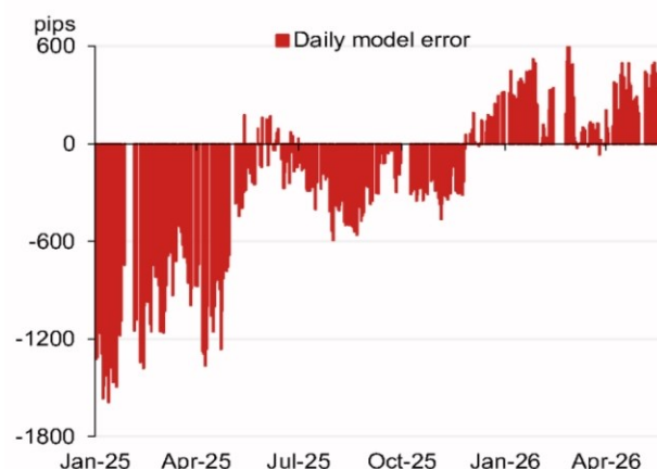
Fig. 2: Recent model errors (without counter-cyclical factor adjustment)
