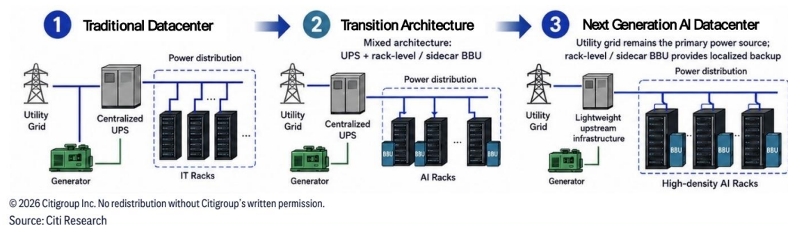
Figure 2 - AI Power Architecture Is Evolving, Making BBU An Increasingly Important Part of Next Gen AIDC We believe AI infrastructure is entering a new power architecture cycle as rack power density continues to increase. Historically, datacenters relied on centralized U
