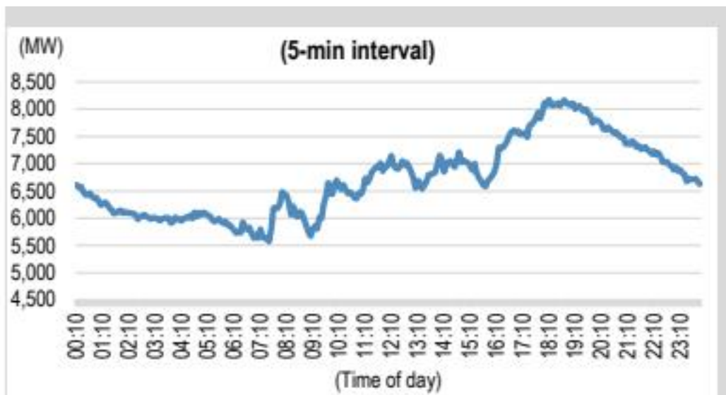
Figure 4 - Figure 4: NSW power load on a typical day Figure 5: Power load by hour in New England on a typical day Figure 6: Power load fluctuations in New England and NSW
