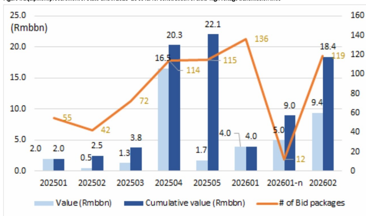
Figure 1. Equipment procurement of State Grid in 2025-26 so far for construction of ultra-high voltage transmission lines
