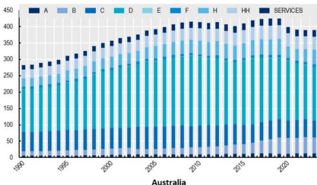
Figure 1 - ## Preliminary results Figure 1. CO 2 emissions with industry/household breakdown Unit: Million tonnes Note: ISIC A “ Agriculture, forestry and fishing ”, B “ Mining and quarrying ”, C “ Manufacturing ”, D “ Electricity, gas, steam and air conditioning supply ”,
