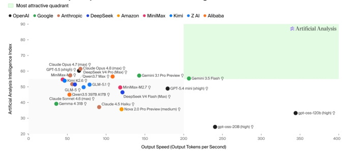
Exhibit 14 - Output speed to run Artificial Intelligence Index as of 8 Jun
