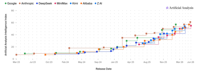
Exhibit 10 - Frontier Language Model Intelligence over time as of 8 Jun
