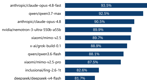
Exhibit 41 - Global: Top 10 models by success rate as of 8 Jun
