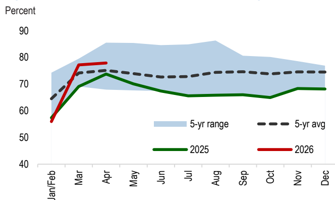
Figure 47: China copper flat-rolled producer operating rates
