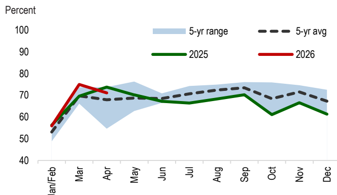
Figure 45: China copper cathode-fed rod producer operating rates
