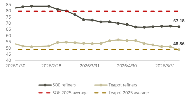
Figure 2: Utilisation of China SOE/teapot refiners
