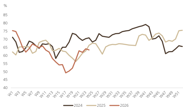
Figure 8: China PDH capacity utilisation
