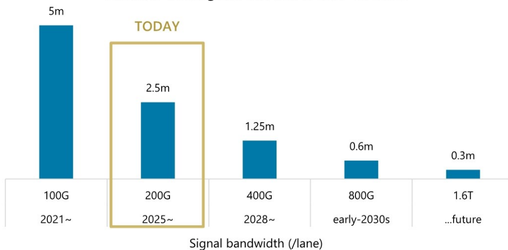
Distance that signals can travel over Cu cable
