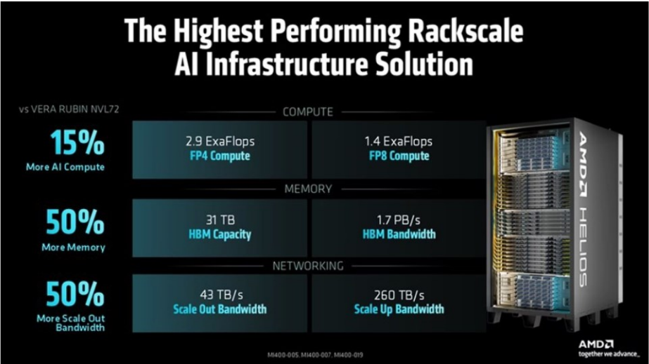
Exhibit 1: AMD Helios Performance Specs
