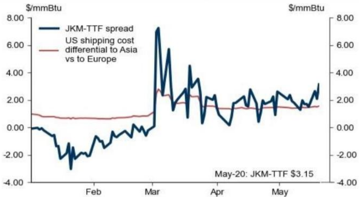
Exhibit 4 - Exhibit 4: The JKM-TTF premium remains strong enough to cover the incremental cost for the US to ship LNG to Asia vs to Europe JKM-TTF spread and the US shipping cost differential (lhs) vs US LNG loadings to Europe vs to Asia, mtpa
