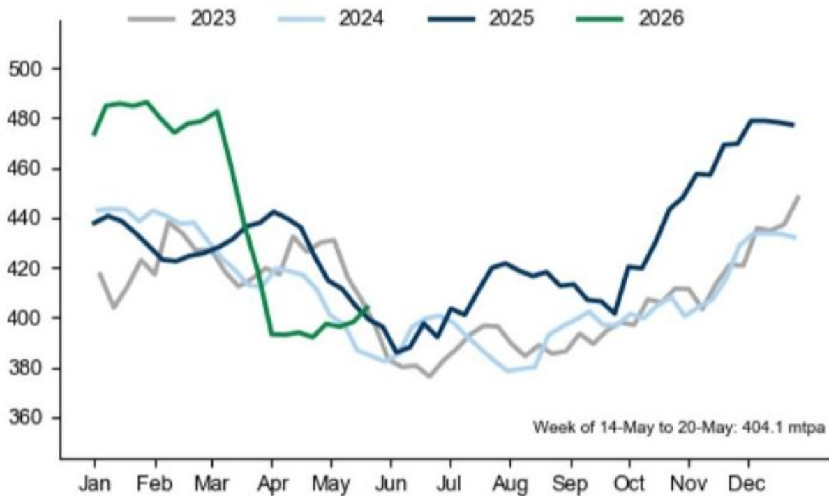
Exhibit 5 - Exhibit 5: LNG loadings are now marginally up yoy as suppliers postpone maintenance... Global LNG loadings, mtpa
