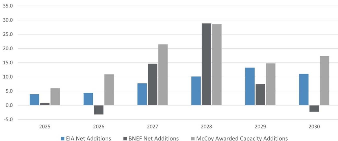
Figure 19: Annual US Gas-Fired Capacity Additions
