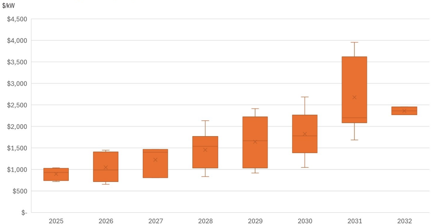
Figure 17: NAM CCGT Project Costs by Completion Date
