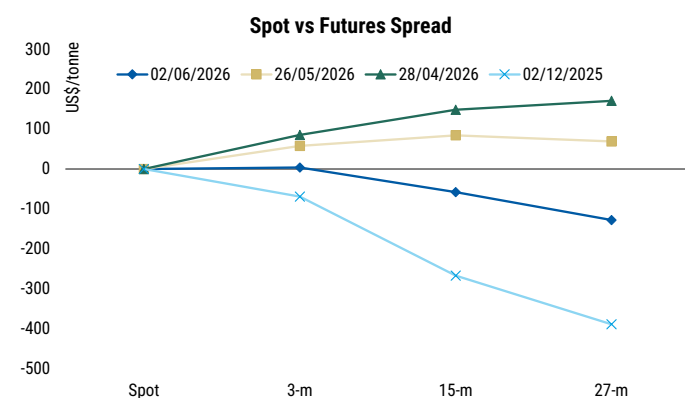
Exhibit 125: Contango vs. Backwardation: Copper Futures Curve Movement
