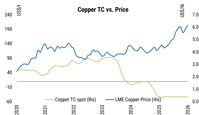
Exhibit 123: Copper Treatment Charges (TCs) vs. Price
