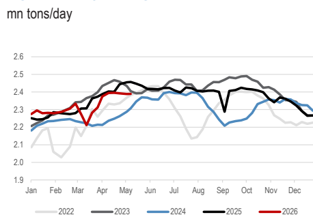
Figure 6: Daily Average Molten Iron Output
