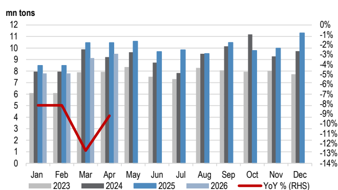
Figure 9: China Steel Products Export Volume
