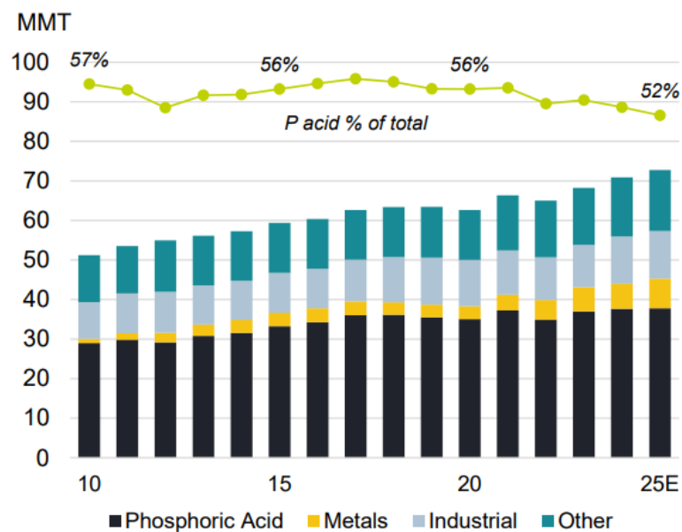
Global Sulphur Demand by Use
