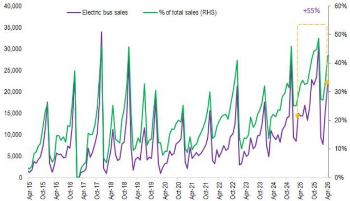
Figure 5 - Figure 5: China electric bus sales LHS: Number of buses sold. RHS: share of of total bus sales
