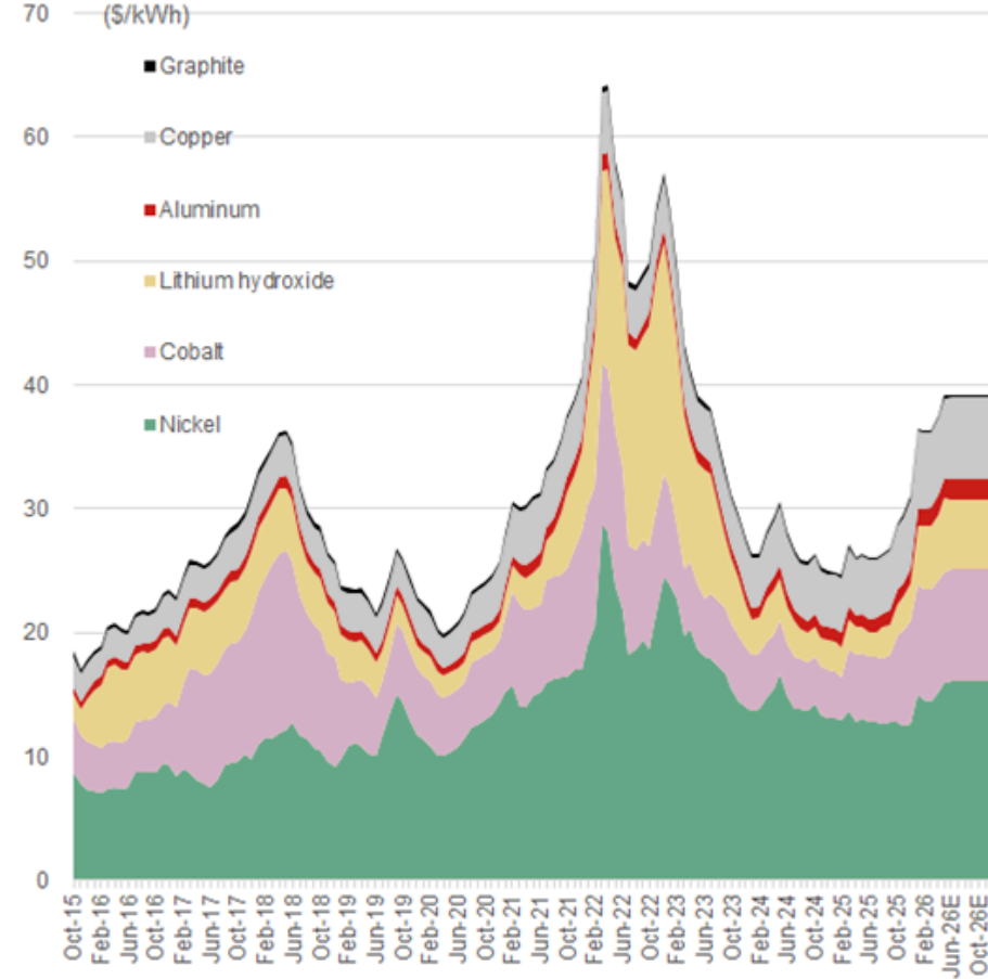
Fig. 82: Estimated input cost per kWh for NCA battery cells (major components)
