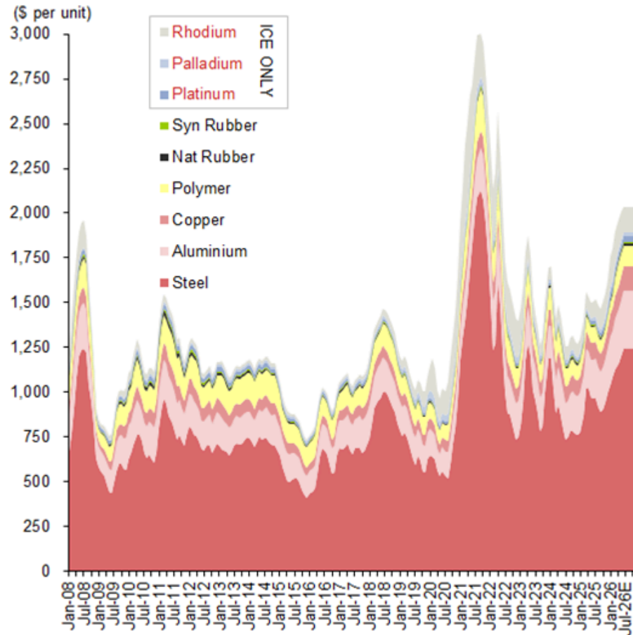
Fig. 81: Estimated input cost per vehicle (global average, including steel)
