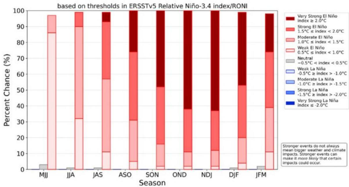
Exhibit 2 - Exhibit 2: NOAA/CPC now assigns a 63% (up from 37%) probability to a very strong El Niño in Nov-Jan, making intensity the key watchpoint NOAA CPC ENSO Strength Probabilities (issued June 2026) based on thresholds in ERSSTv5 Relat
