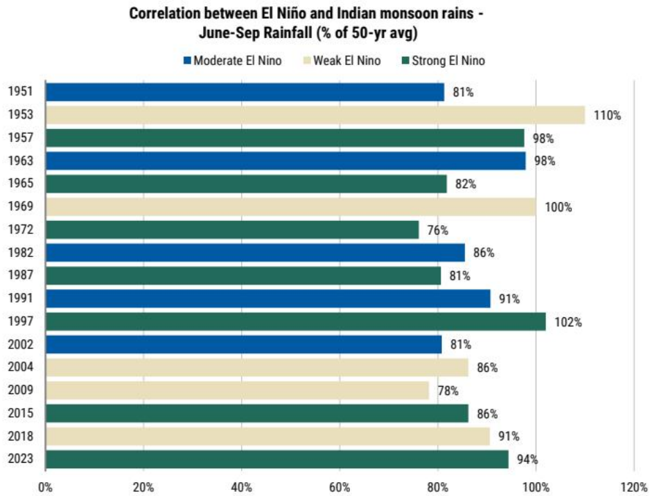
Exhibit 12 - Exhibit 12: India usually receives below-normal rainfall during El Niño years. India is the world second largest sugar producer and below normal monsoon may reduce its sugar output potential Correlation between El Niño and Indian
