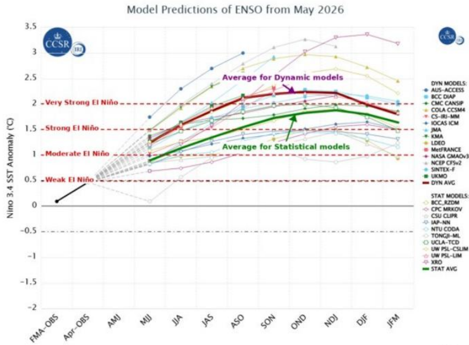
Exhibit 4 - Exhibit 4: El Niño is now confirmed, while very-strong odds increased to 63% in Nov-Jan from 37% in the prior update Exhibit 5: El Niño strength distribution remains wide
