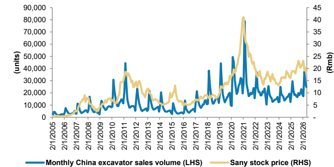
Exhibit 2: China's monthly excavator sales volume vs. Sany Heavy's share price
