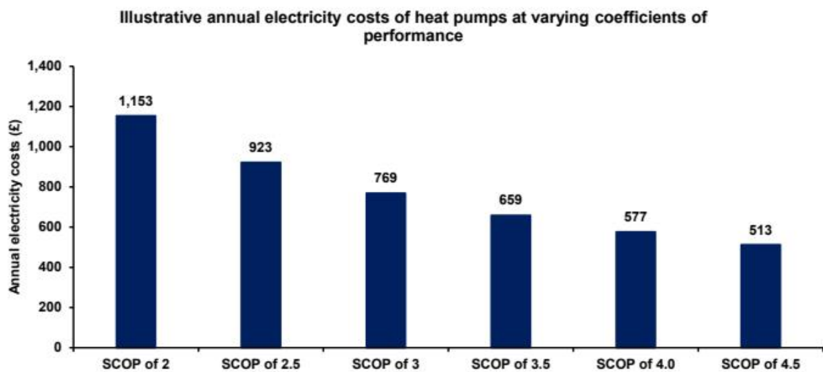
Exhibit 8 - EXHIBIT 8: Achieved operating efficiency is a key driver of the total cost of ownership for a heat pump
