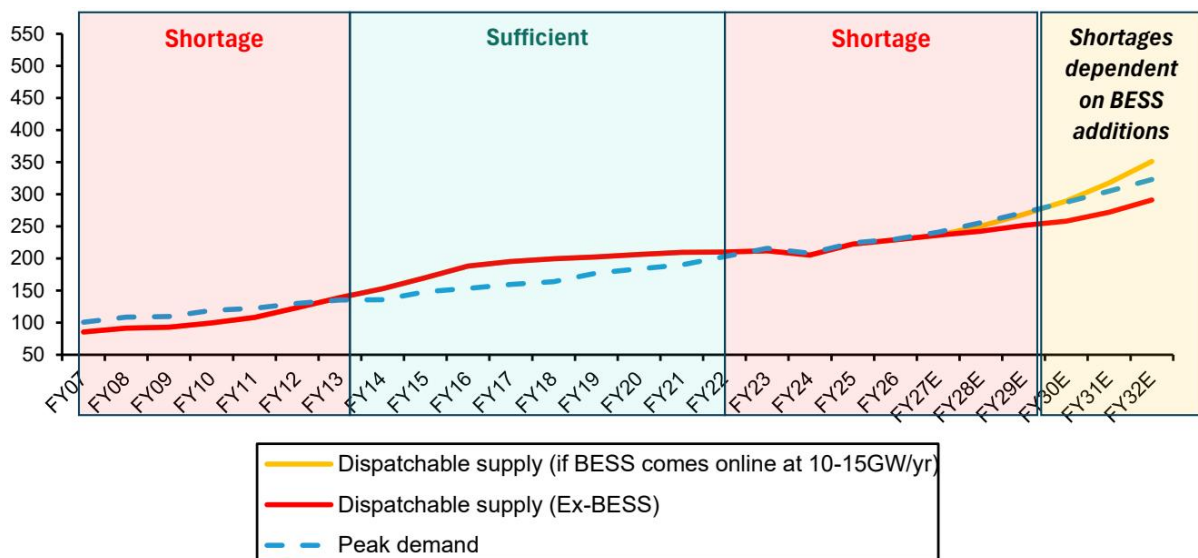
EXHIBIT 14 - EXHIBIT 14: Power demand-supply: We see power shortages continue next 3 years, and a need for 15 GW/yr of BESS to reduce the gap... India - Peak Demand-Supply (GW)
