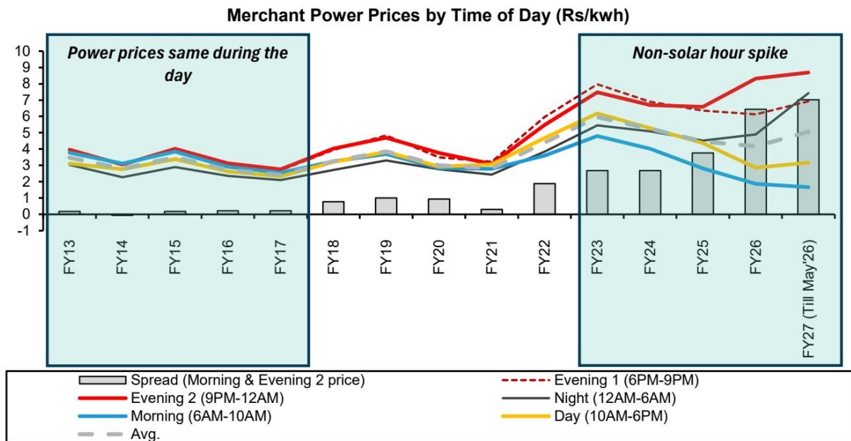
EXHIBIT 5 - EXHIBIT 5: Spot power prices: While overall spot prices have come down, evening continues to be high, and also the day-evening arbitrage is increasing
