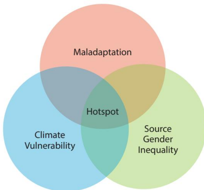
Figure 1 - Figure 1: Climate Vulnerability, Gender Inequality, and Maladaptation in Southeast Asian Agriculture Creates a Self-Reinforcing Hotspot ## QUANTIFYING THE DUAL CONSTRAINT ## Climate Vulnerability and Agriculture
