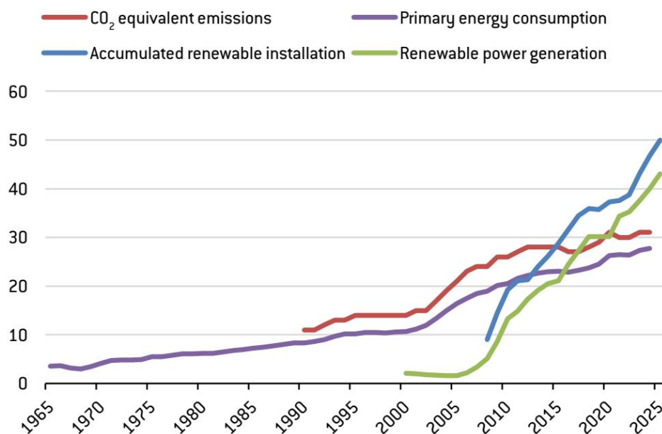
Figure 2 - Figure 1: China's share of global emissions and energy (%) Figure 2: Chinese domestic energy production as a share of demand (%)
