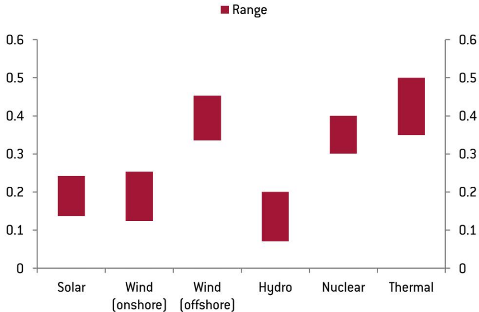
Figure 3 - Figure 3: Levelised cost of power generation by energy
