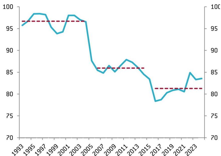
Figure 2 - Figure 1: China's share of global emissions and energy (%) Figure 2: Chinese domestic energy production as a share of demand (%)
