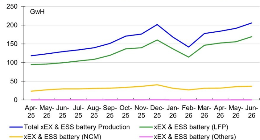
Figure 5: China xEV and ESS battery production volume trend by product
