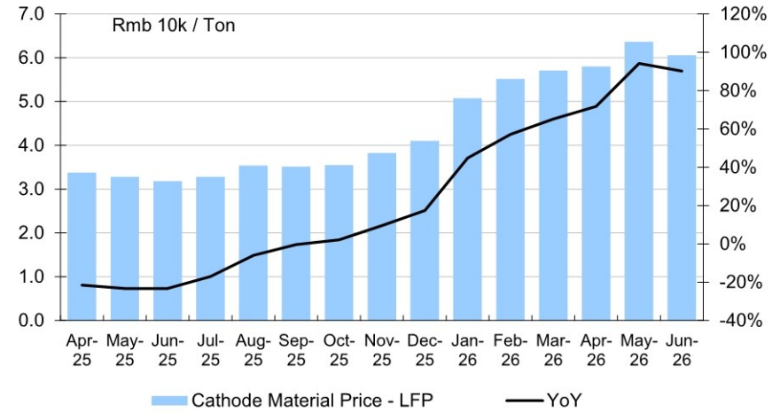
Figure 33: Cathode material LFP price trend
