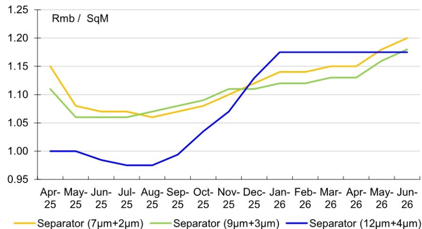
Figure 38: Separator price trend by product
