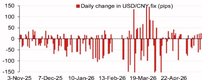
Fig. 3: Daily change in USD/CNY fix
