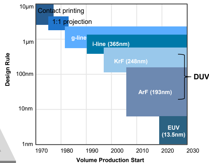
History of shorter-wavelength exposure light sources as feature sizes shrink
