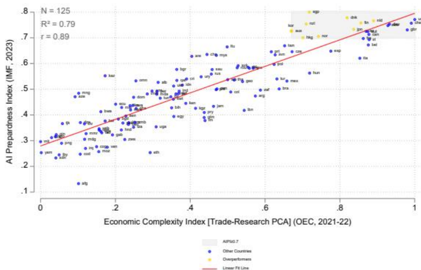
Figure 3 - Figure 3: Global relationship between AIPI and ECI a) Unweighted analysis b) Population-weighted analysis Both charts highlight the top performers in AI preparedness, concentrated in the northeast quadrants. Consistent with pr
