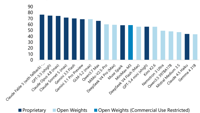
Exhibit 22 - Coding index for top 20 models as of 6 Jul
