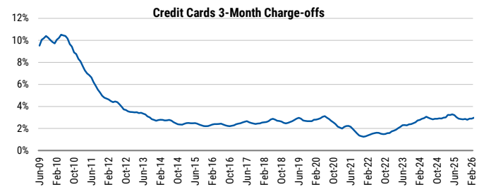
Exhibit 65: 3-month charge-offs
