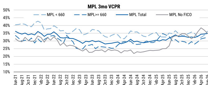
Exhibit 52: 3-month VPCR
