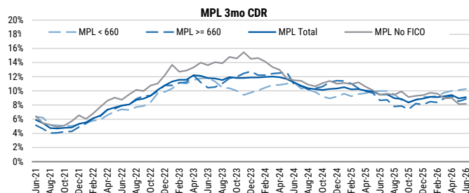
Exhibit 51: 3-month CDR
