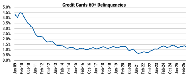
Exhibit 62: 60+ delinquencies
