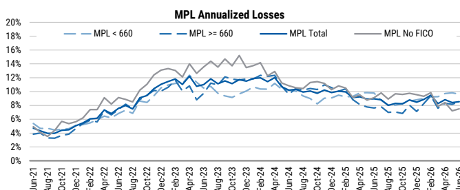
Exhibit 53: Annualized losses
