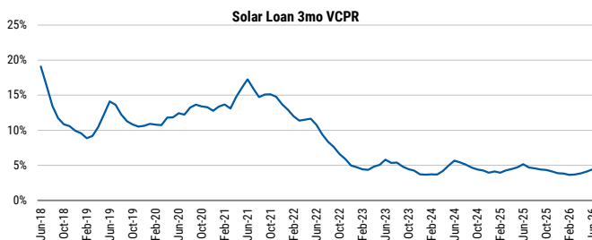
Exhibit 68: 3-month VCPR
