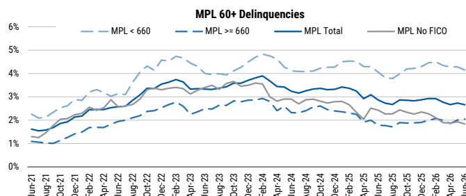
Exhibit 50: 60+ delinquencies
