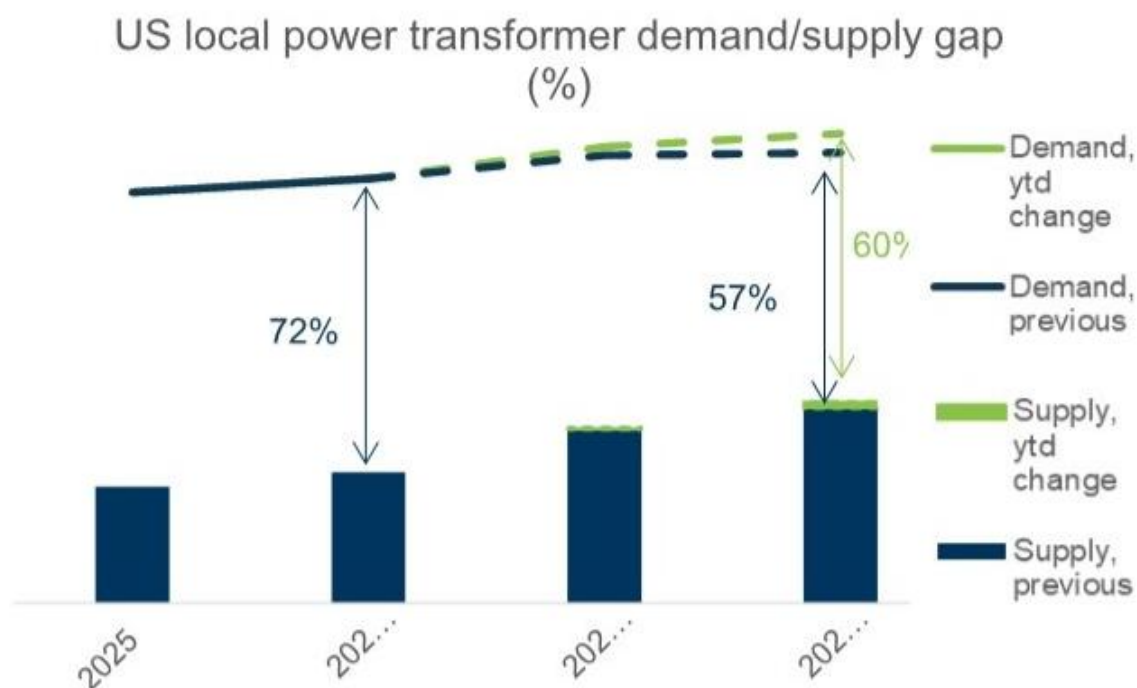
Exhibit 1 - Exhibit 1: We continue to estimate that US power transformer demand/local supply gap would narrow from 72% to 60% in 2028E; while US PPI has stabilized at a high level, China export price is up +23% yoy (Feb-Apr avg, for 2
