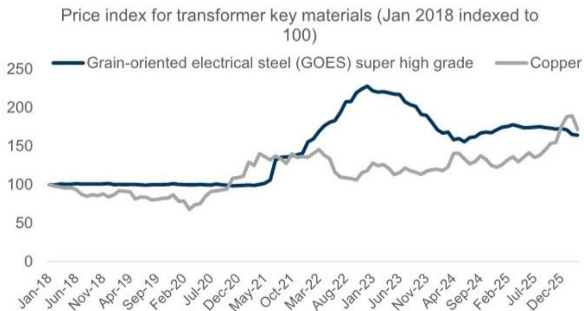
Exhibit 8 - Exhibit 8: Key raw materials for transformer, GOES, saw prices inch down, while copper price had a sharp increase in 4Q25, and dipped in March 2026
