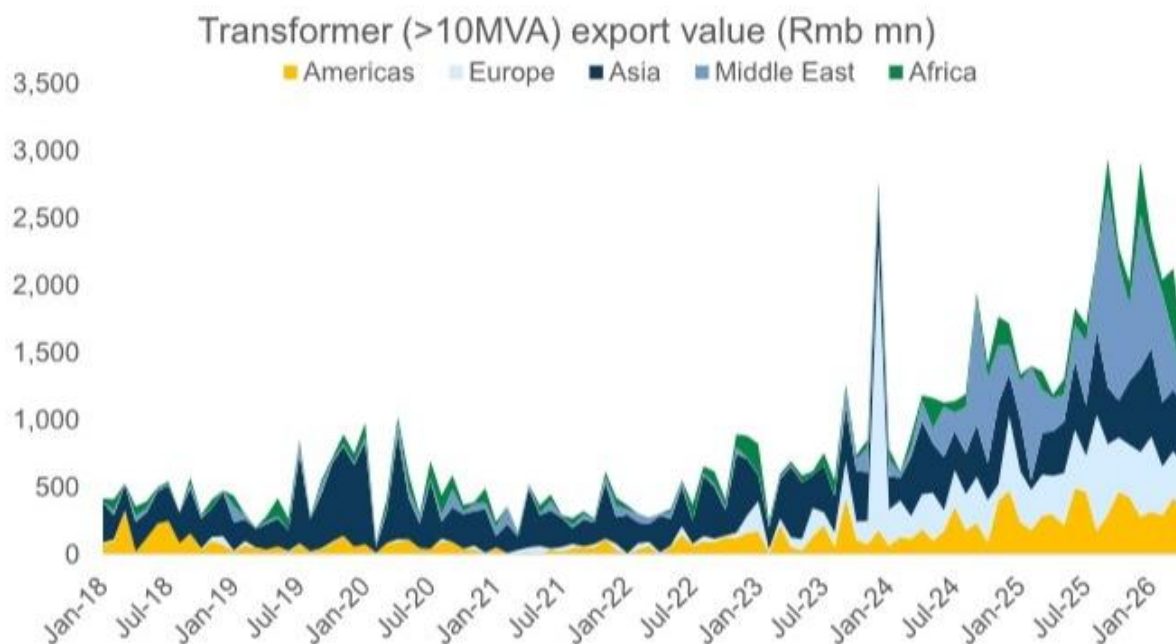
Exhibit 2 - Exhibit 2: China total transformer export value grew 27% in April (slowing vs 56% in March) Exhibit 3: China transformer export value to the US grew +95% yoy in April (vs 118% yoy in March)
