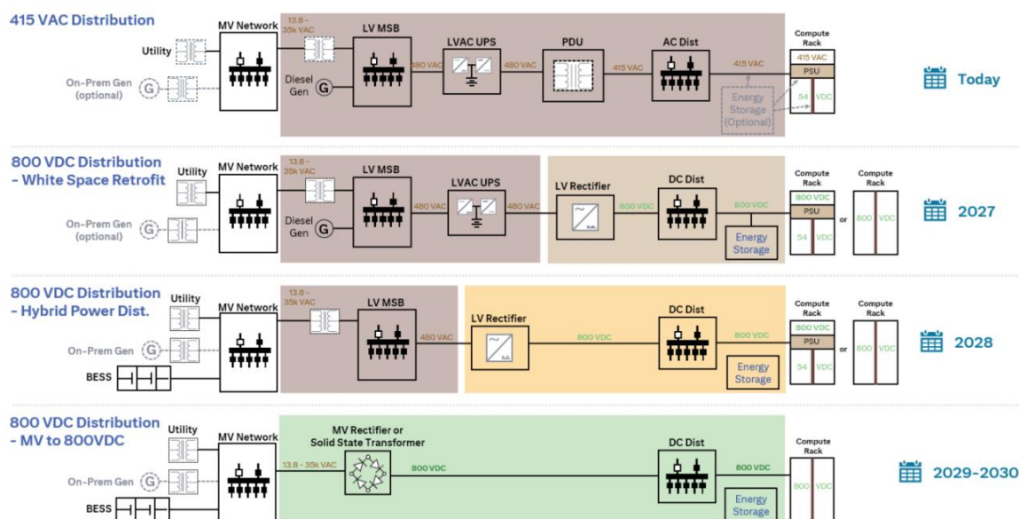
Figure 1 - # Nvidia's 800VDC Architecture: Four Generations, from Multi-Stage AC to a Single Integrated DC Conversion NVIDIA's reference architecture defines 4 generations of data center power distribution, each representing a step-change reduction in conversion stages (
