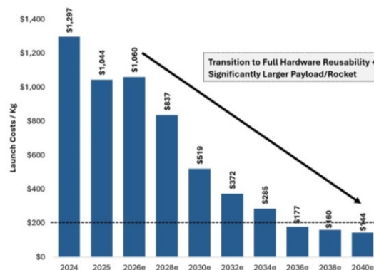
Projected SpaceX Launch Costs/Kg Over Time
