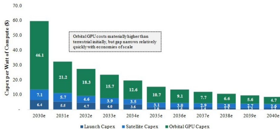
Capex per Watt for Orbital Compute
