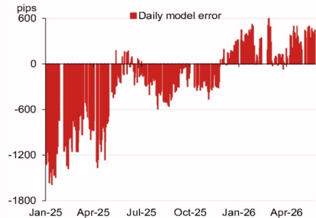
Fig. 2: Recent model errors (without counter-cyclical factor adjustment)
