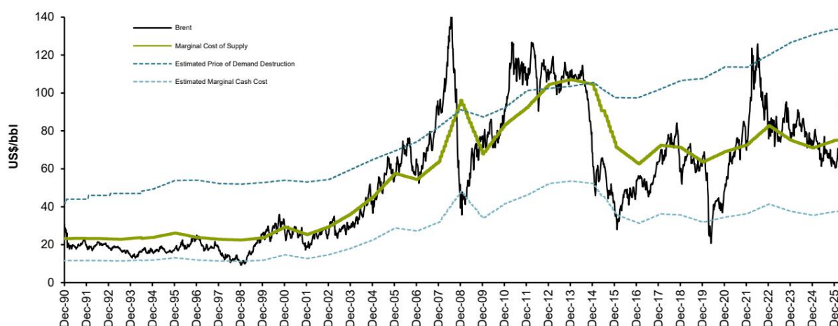
EXHIBIT 2 - EXHIBIT 2: The Marginal Cost of Oil for Top 50 decreased by 2% to US$69/bbl in 2025
