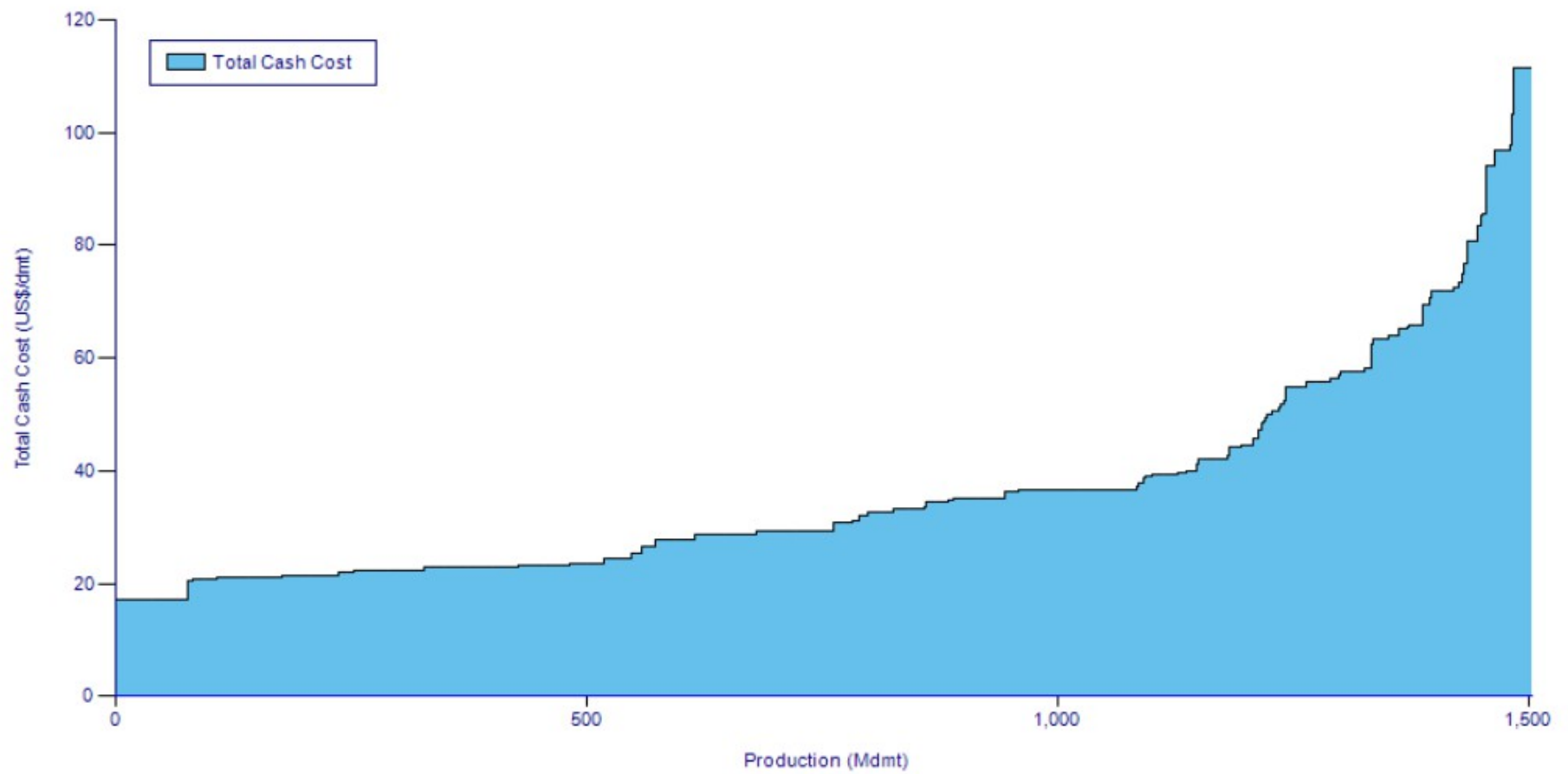
Figure 49: Seaborne iron ore cost curve – 2025
