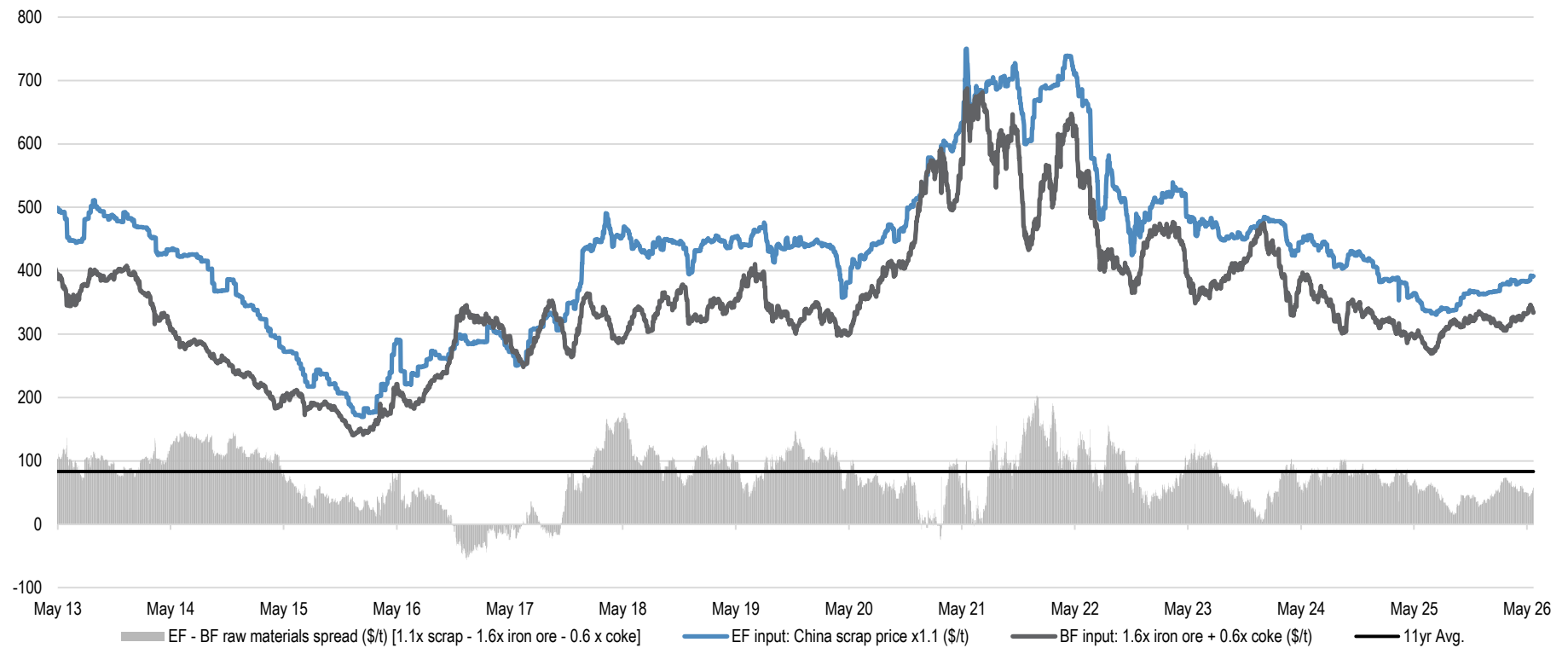
Figure 39: Blast furnace vs electric furnace raw material costs ($/t)
