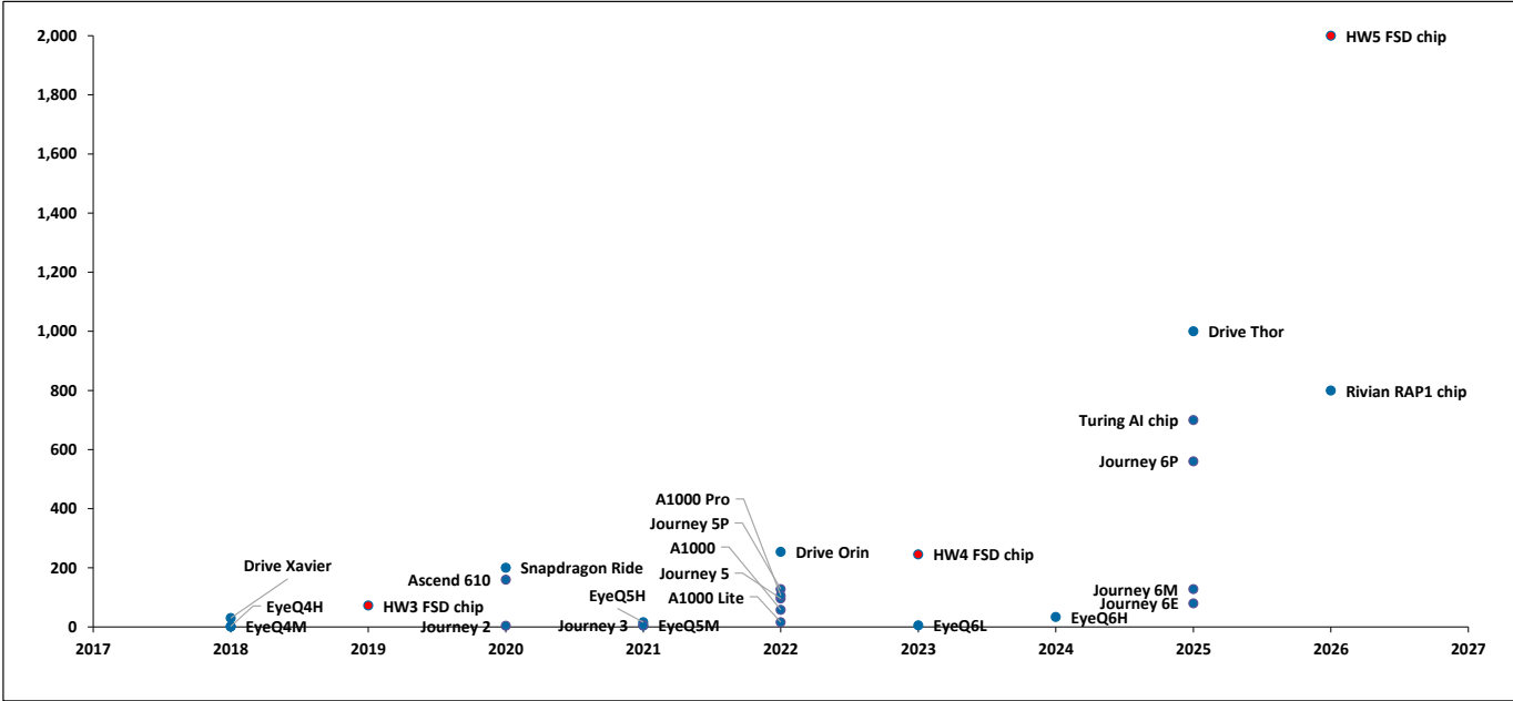
Figure 4: Estimated Compute for Key Autonomous Vehicle Systems
