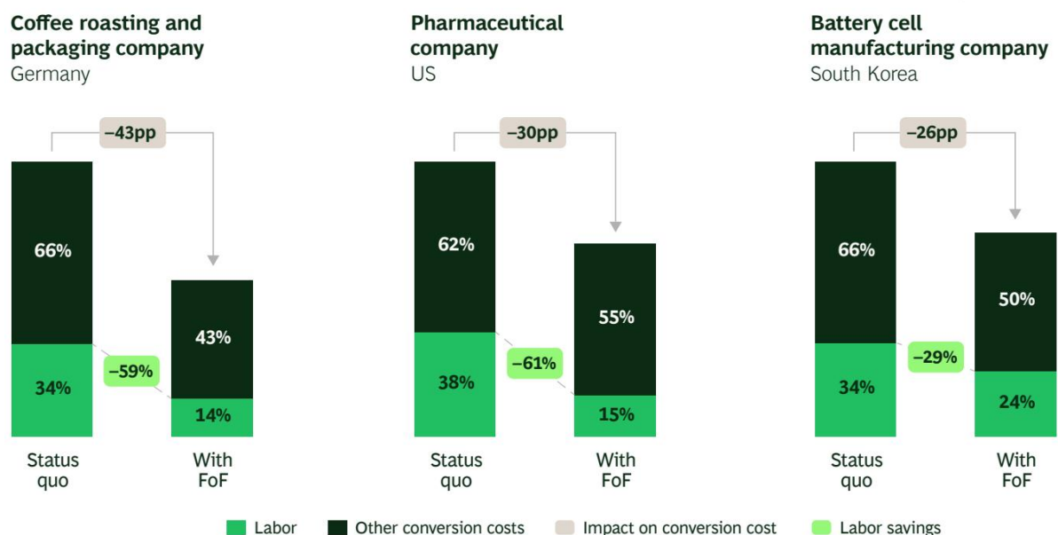
EXHIBIT 1 - ## EXHIBIT 1 How the Factory of the Future Significantly Lowers Conversion Costs Coffee roasting and packaging company Germany Note: FoF = Factory of the Future. Other conversion costs include cost of energy, depreciation costs, and other operational expenditure
